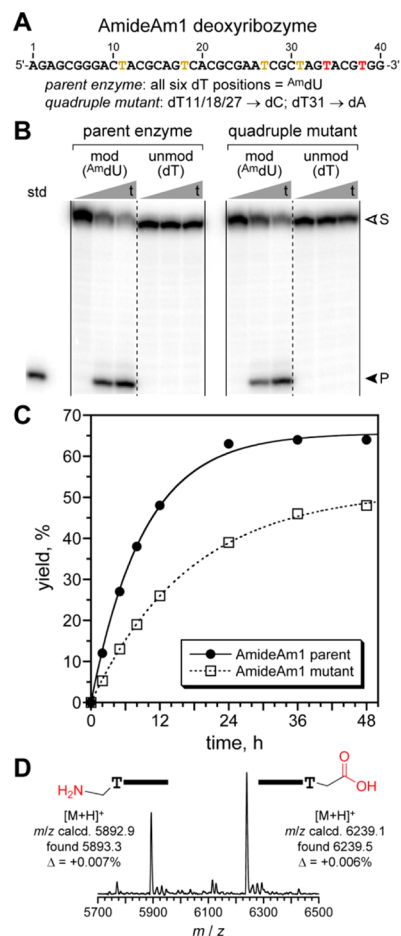
Figure 2. AmDU-modified AmideAm1 deoxyribozyme for amide hydrolysis. (A) Sequence of the initially random (N 40 ) region of AmideAm1. The four yellow T positions are AmDU in the parent sequence but mutable as indicated. (B) PAGE assay ( t = 0, 12, 48 h). (C) Kinetic plots. k obs h -1 ( n = 3): parent 0.11 ± 0.01 and quadruple mutant 0.057 ± 0.007. Because k bkgd < 10 -4 h -1 (i.e., <0.5% in 48 h), the rate enhancement k obs / k bkgd is >10 3 . (D) Mass spectrometry analysis of AmideAm1 product.
