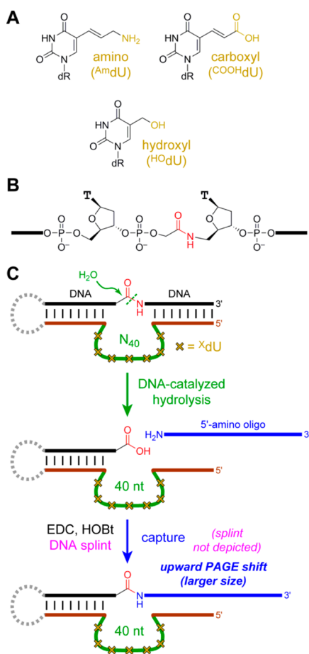
Figure 1. In vitro selection using modified DNA to achieve amide hydrolysis. (A) Modified X dUTP nucleosides used in this study (dR = deoxyribose). (B) Amide substrate. (C) Key steps of in vitro selection, in which DNA-catalyzed amide hydrolysis is followed by DNA-splinted capture of the revealed carboxylic acid with a 5'-amino oligonucleotide. The DNA modifications in the initially random (N 40 ) region are denoted schematically by yellow crosses. Not depicted is PCR after the capture step to form the reverse complement of the captured DNA sequences (without modified X dU), followed by primer extension (with modified X dUTP) to synthesize the DNA pool for the next round, now enriched in catalytically active sequences. See SI text and Figure S1 for selection details.
